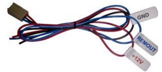
Fig.4. Power cable
