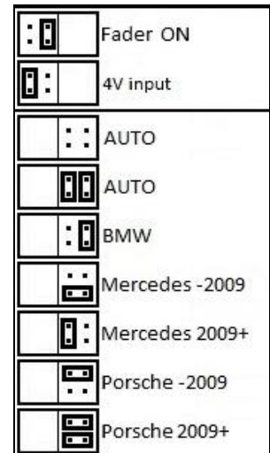
Fig.7. Jumper settings
