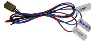
Fig.4. Power cable
